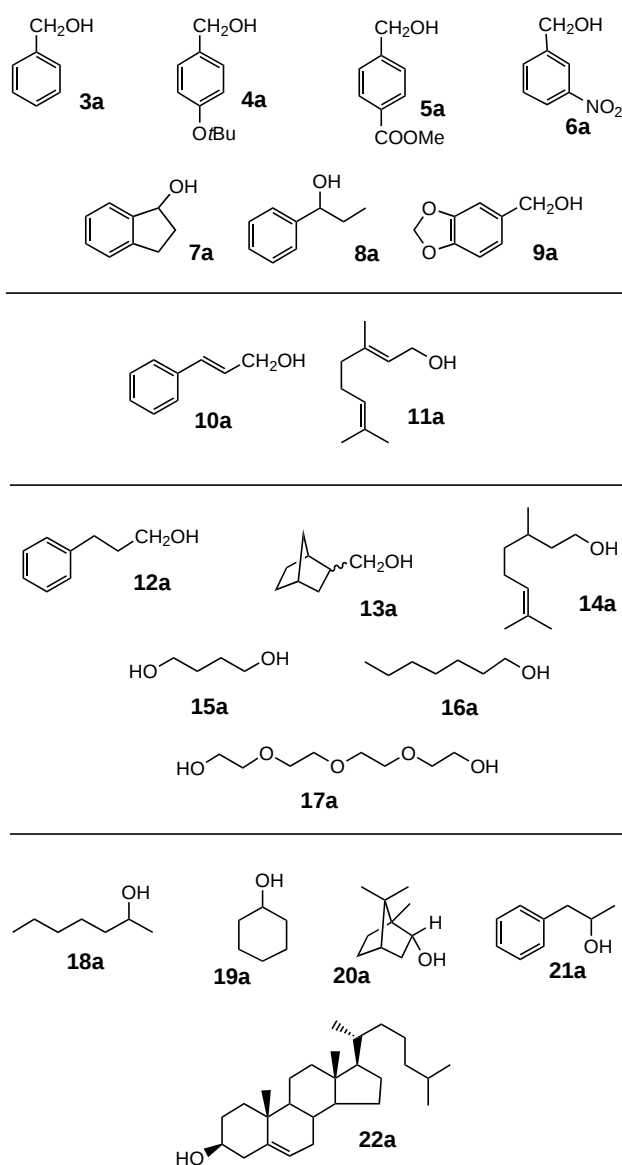
Scheme 1. Oxoammonium resin 2 was prepared in a three-step procedure from chloromethylated polystyrene resin and was employed in the oxidation of alcohols 3a–22a . Oxidation of resin 1 was effected by \text{Br}_2 , \text{Cl}_2 , or \text{NCS/HCl} (Methods A–C).
